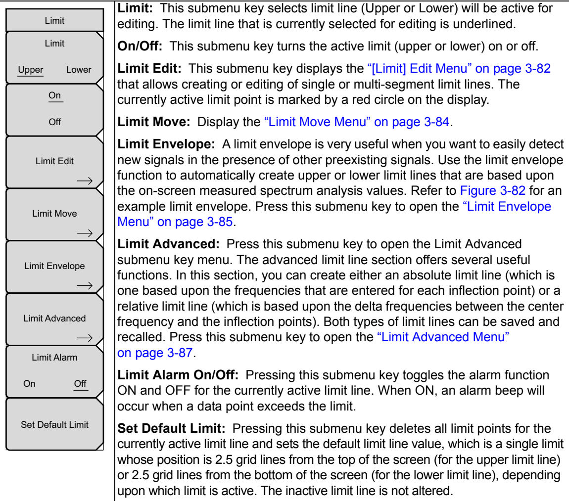
Figure 3-77. IA Limit Menu
