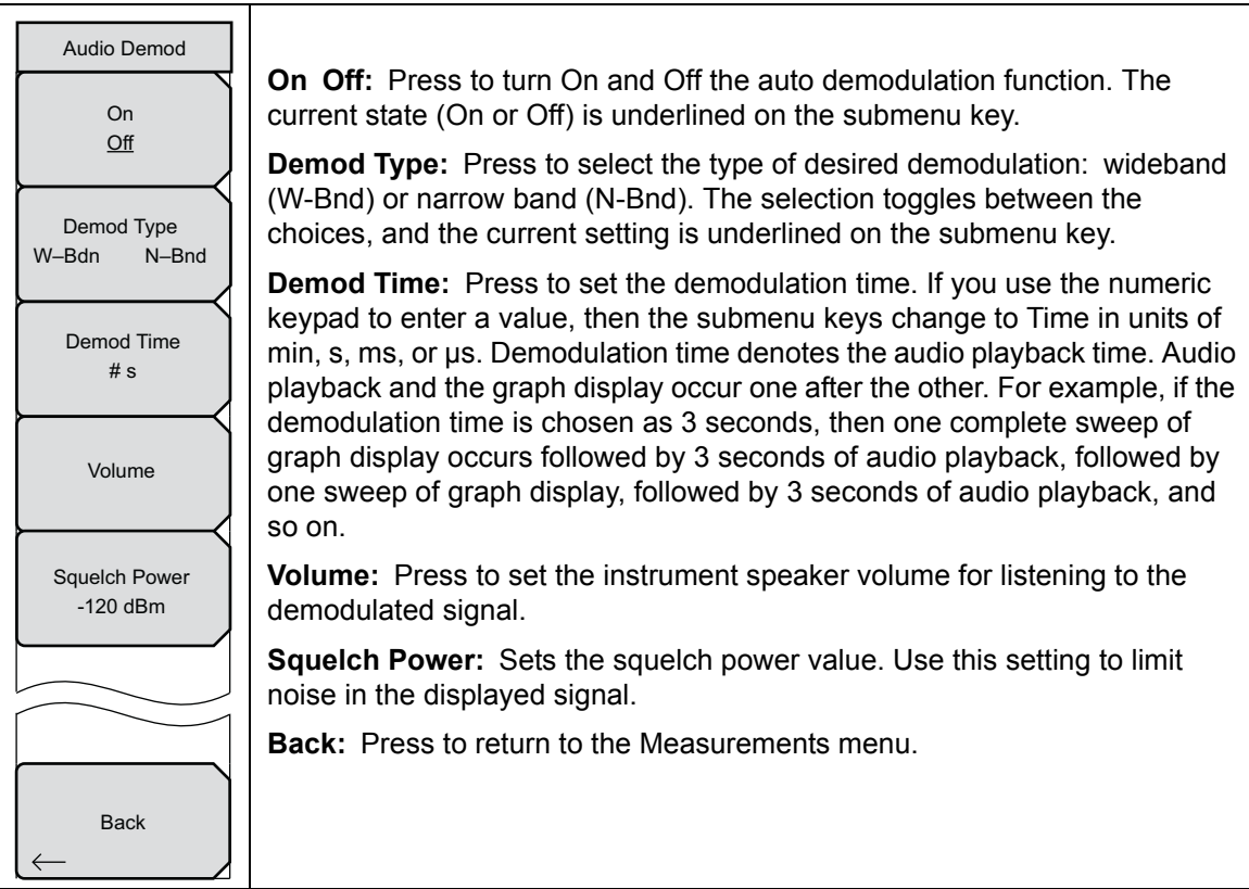
Figure 7-27. Auto Demod FM Menu
