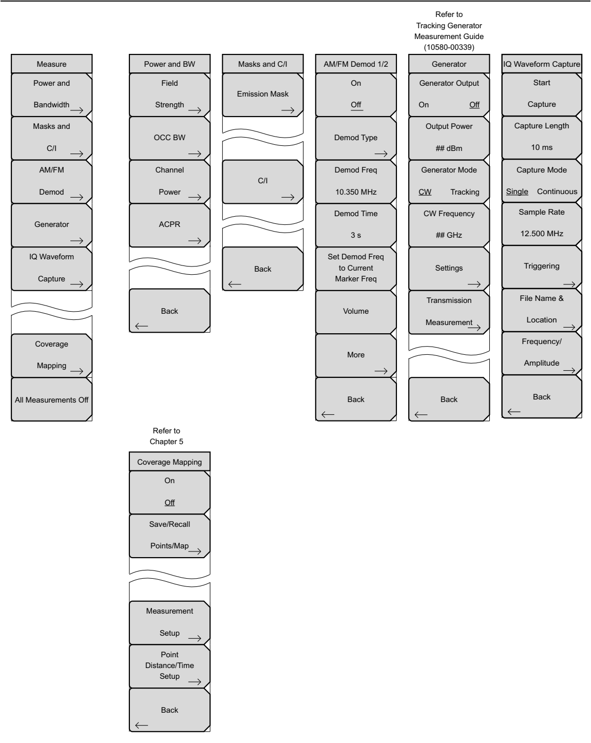
Figure 2-16. Measure Submenu Keys — Measure
