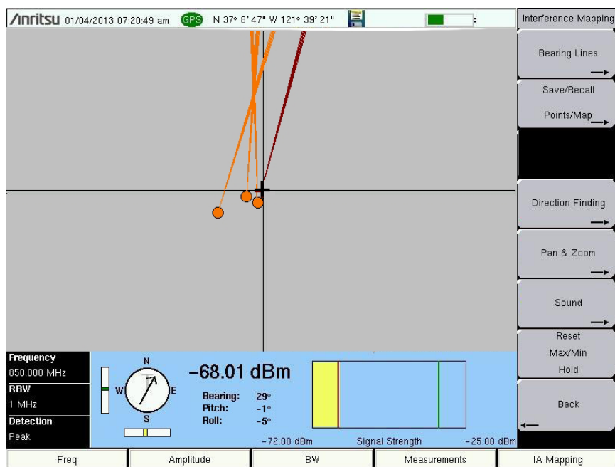
Figure 3-9. Locating an Interfering Signal with the MA2700 and the Default Grid
