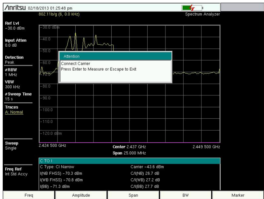
Figure 2-8. C/I Measurement, Ready to Measure the Carrier
