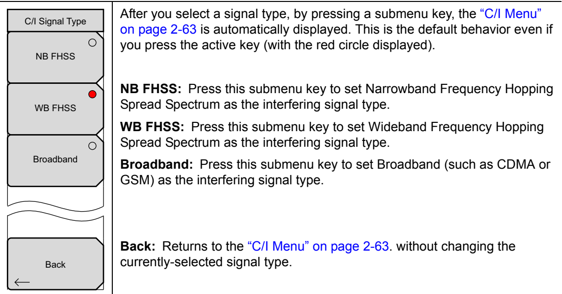
Figure 2-52. C/I Signal Type Menu
