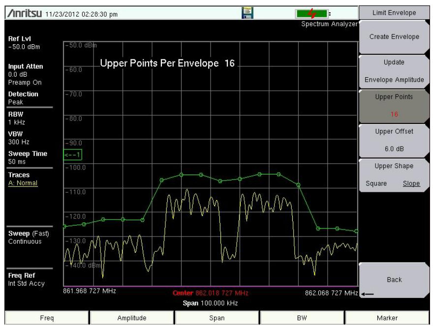
Figure 2-72. Sloped Limit Envelope
