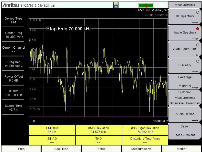
Figure 7-1. Audio Spectrum
