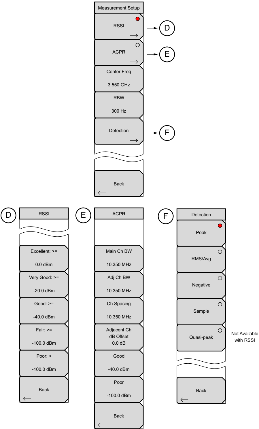
Figure 6-7. Coverage Mapping Menu Keys (Part 2)
