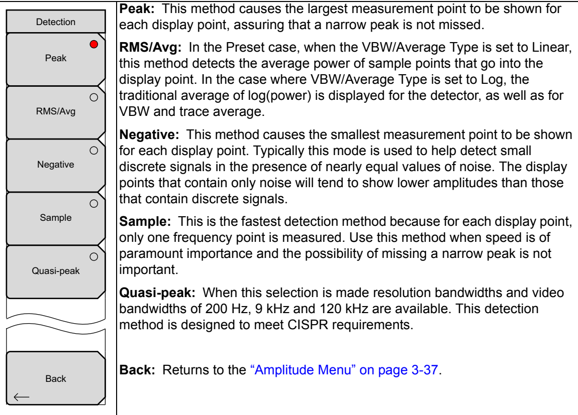
Figure 3-32. IA Detection Menu
